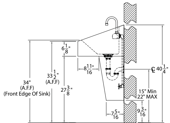
7-PS-41 & 7-PS-46 Hand Sink W/ Front Loading Towel Dispensing
