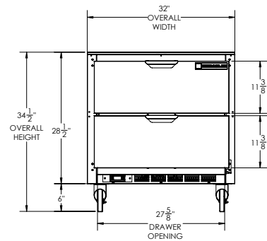
ELEVATION VIEW
