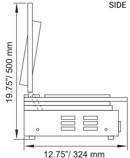
SIDE
