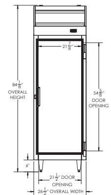
ELEVATION VIEW
