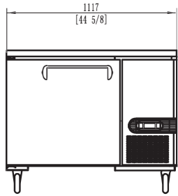
C-RWT44-HC
