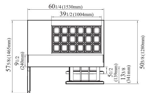
TST-60SD-18M-D2L-FB-N-LW TOP VIEW
