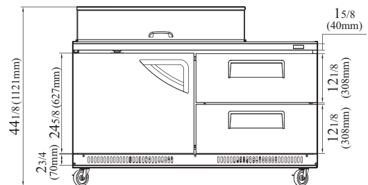
TST-60SD-18M-D2L-FB-N FRONT VIEW
