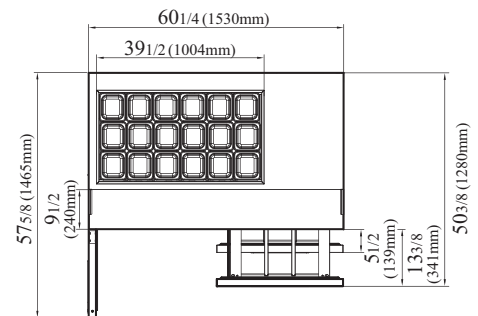
TST-60SD-18M-D2L-FB-N TOP VIEW
