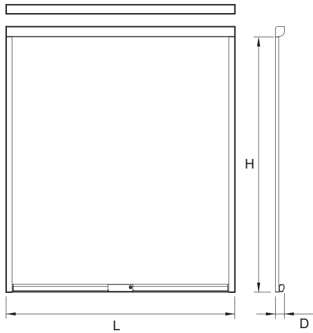
SC-E Plan View
