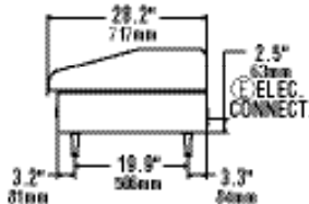
All Models [Right Side View]
