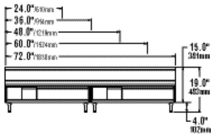
All models [Front View/Elevation] Width varies with model
