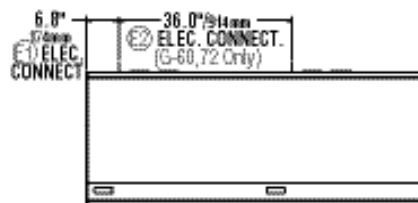
All Models [Top View/Plan] LGC-60, LGC-72 require 2 E connections
