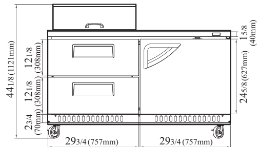
TST-60SD-12M-D2R-FB-N FRONT VIEW
