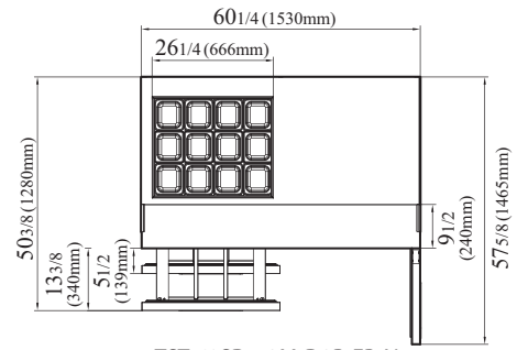
TST-60SD-12M-D2R-FB-N TOP VIEW
