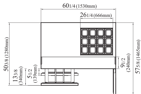
TST-60SD-12M-D2R-FB-N-LW TOP VIEW
