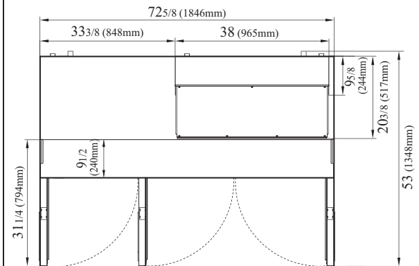
TST-72SD-10S-N-CL-LW
