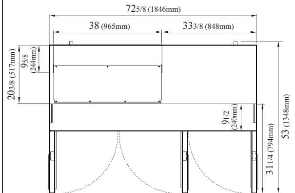
TST-72SD-10S-N-CL
