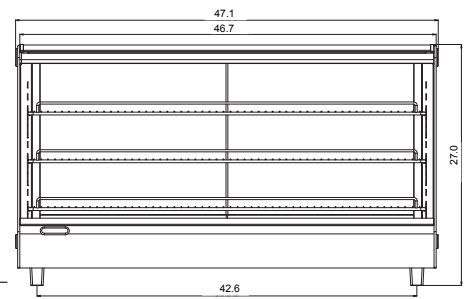
C-HCT47 BACK VIEW
