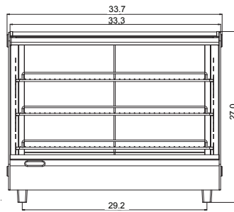
C-HCT34 BACK VIEW
