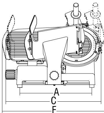
Tilt-carriage with zero blade exposure
