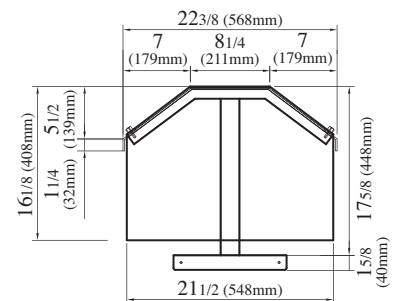
STAND SIDE VIEW
