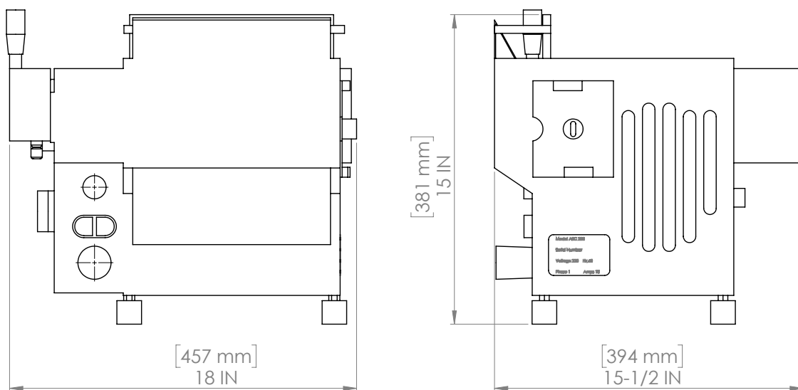
ASC250 DIMENSIONS
