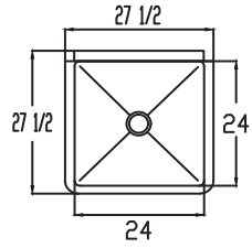
BSP-24-14
