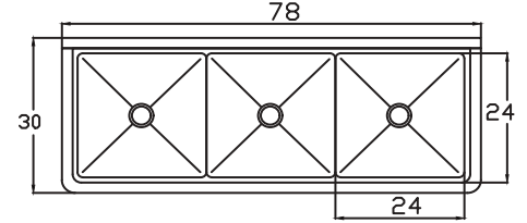
BS3-24-14/N
