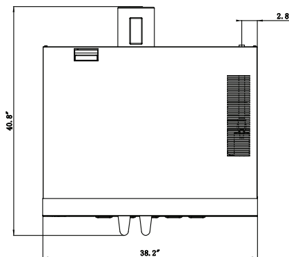
SIDE VIEW - DOUBLE
