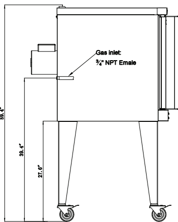
SIDE VIEW - SINGLE
