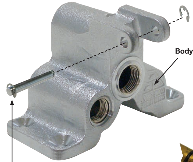
Pedal Mounting Pin with Clips
