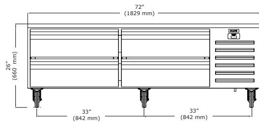
Front (72" Model)
