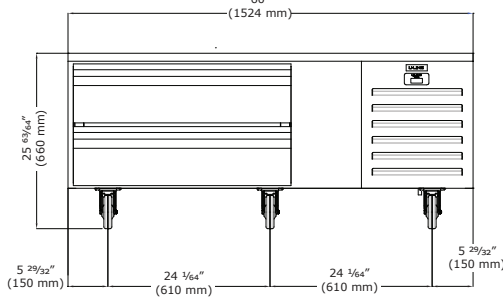
Front (60" Model)
