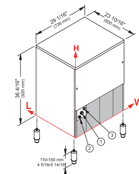
Adjustable feet 4 5/16" – 5 14/16"
