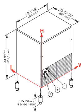
Adjustable feet 4 5/16" – 5 14/16"
