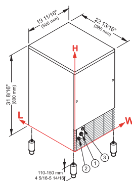
Adjustable feet 4 5/16" – 5 14/16"
