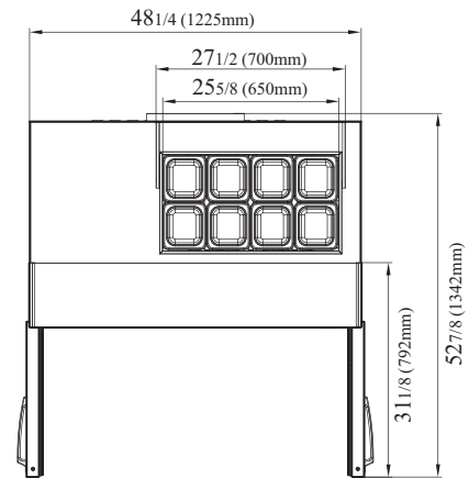
PST-48-08S-N-LW TOP VIEW
