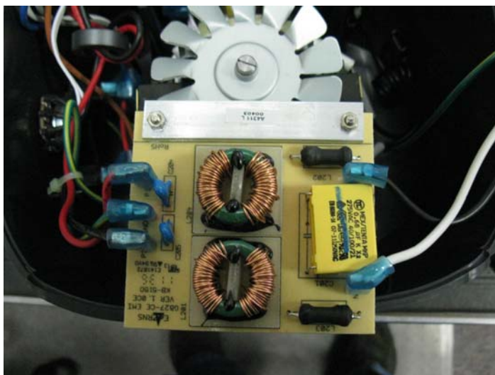
Figure 4. RFI Board
