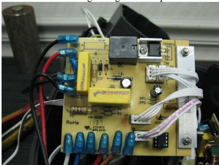
Figure 3. PC Board
