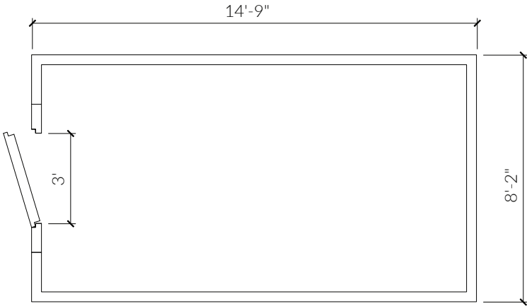
FWF8X15-1A
