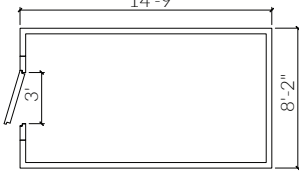
FWF8X15-1B 14'-9"
