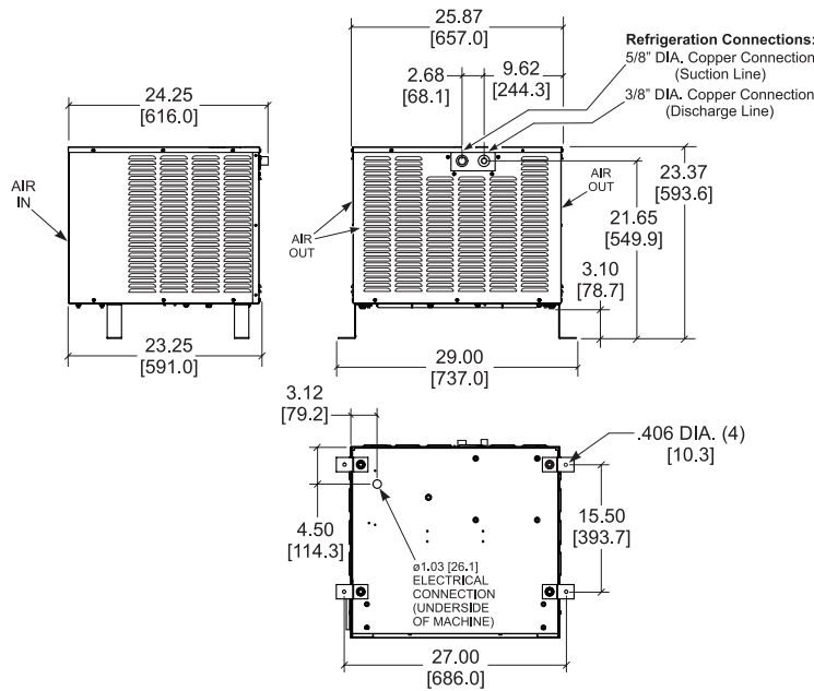
FIGURES IN BRACKETS INDICATE MILLIMETERS / DECIMAL AND FRACTIONAL DIMENSIONS EQUAL TO ( PLUS OR MINUS 1/16 INCH [1.5mm] ).
