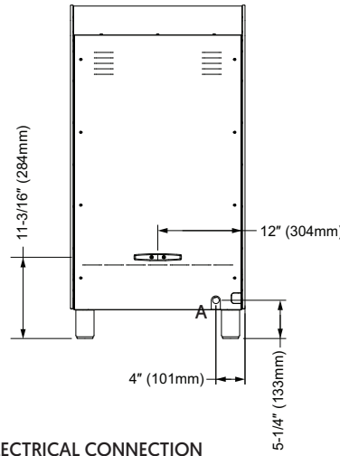
A: ELECTRICAL CONNECTION
