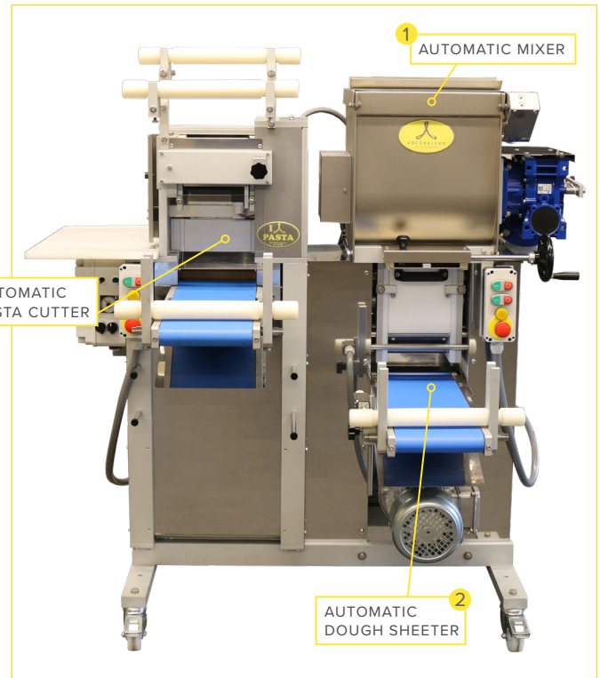
MIXER
