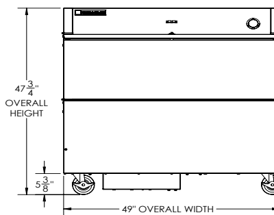
ELEVATION VIEW
