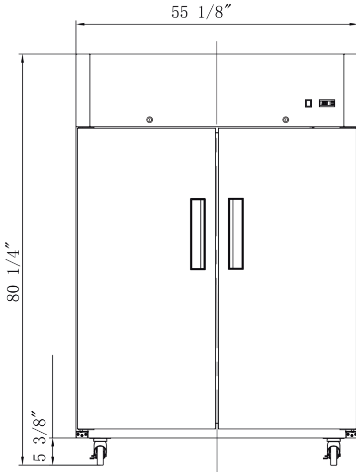
Front View
