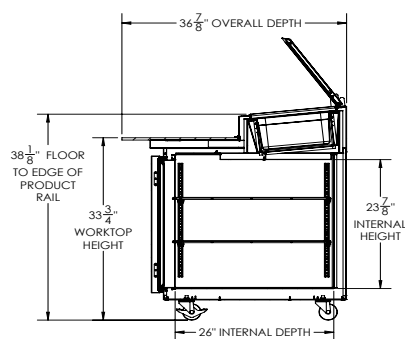
ELEVATION VIEW
